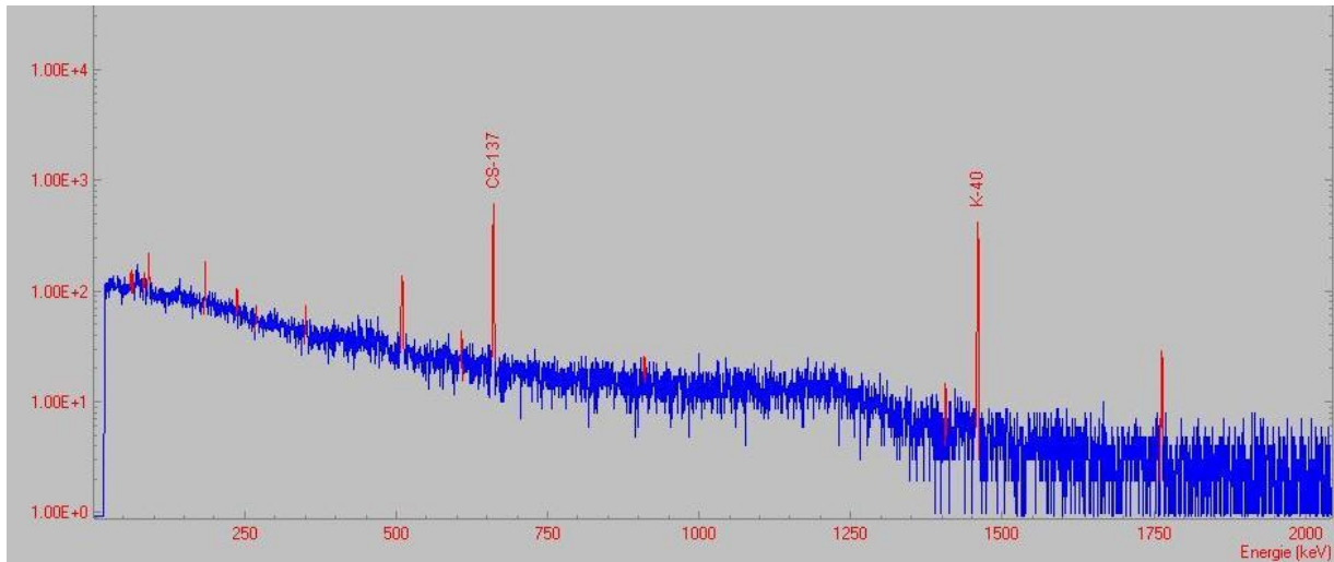
Fig.4: Typical \gamma -spectrum of a mushroom sample contaminated with Cs-137
