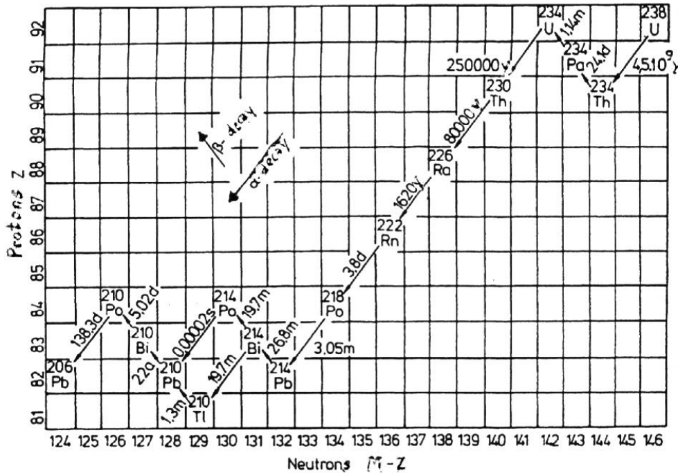
Fig.2: Natural decay chain of ^{238}\text{U} with half-lives of the descendants (d days; m minutes; s seconds; y years)
