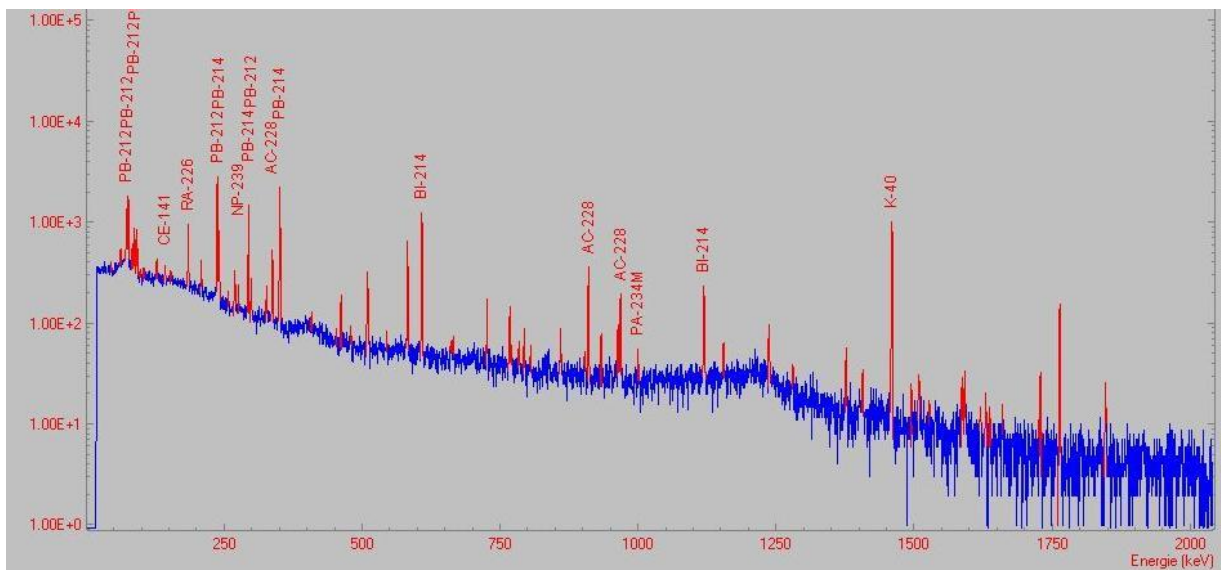
Fig.5: \gamma -spectrum of construction material containing natural uranium
