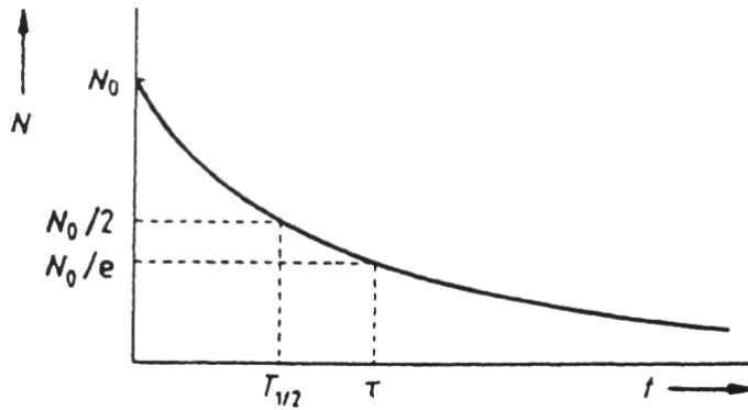
Fig.1: The course of the radioactive decay
